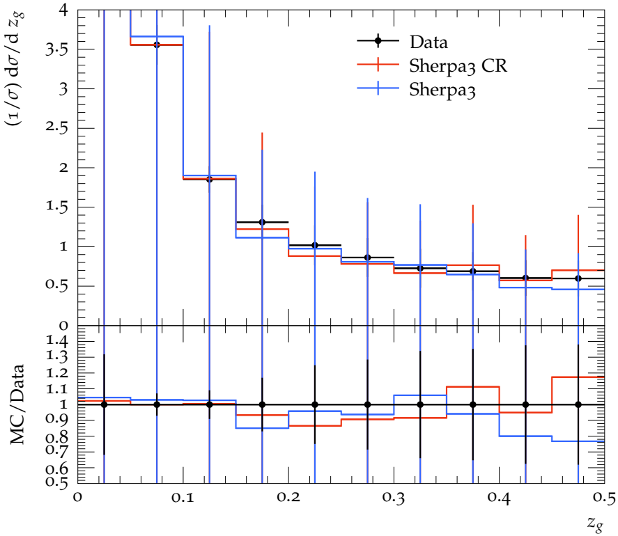
Dijet selection, Gluon extraction, Track Based, Soft Drop \beta = 2.0 , z_g
