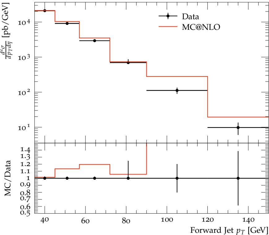
Measurement of forward+central jets at \sqrt{s} = 7 TeV
