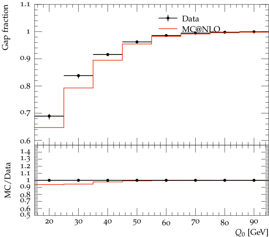
Gap fraction as a function of Q_0 for events satisfying 2 < \Delta y \leq 3
