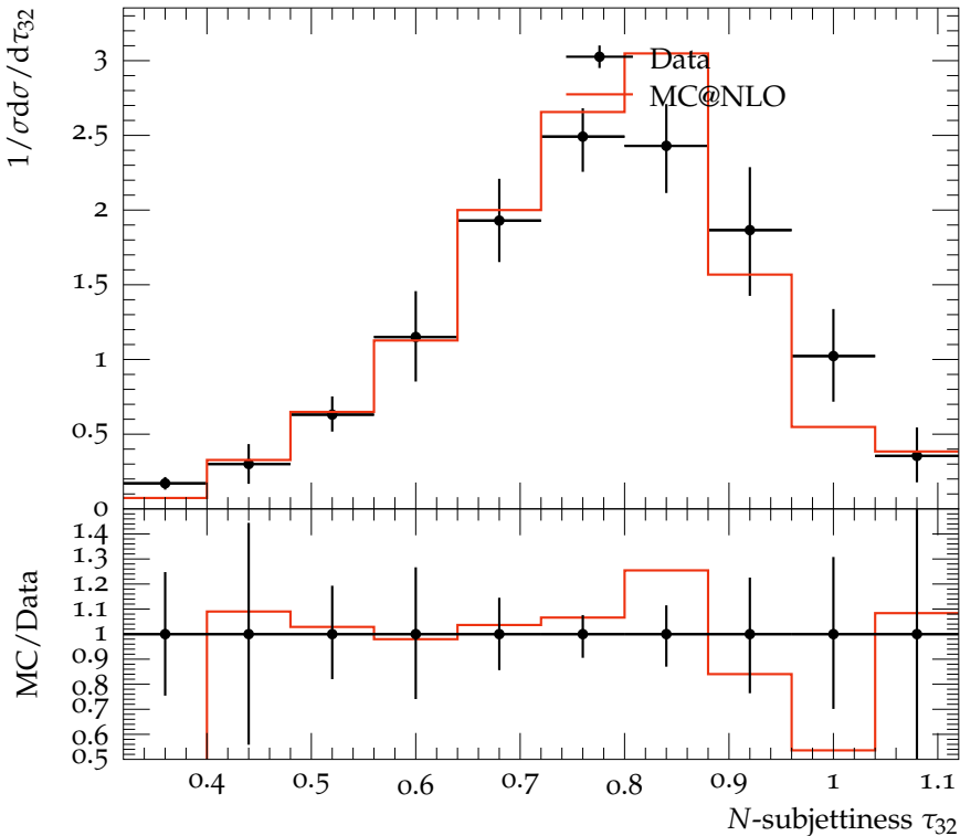
Cambridge-Aachen jets, R=1.2 , 500 \text{ GeV} < p_{\perp} < 600 \text{ GeV}
