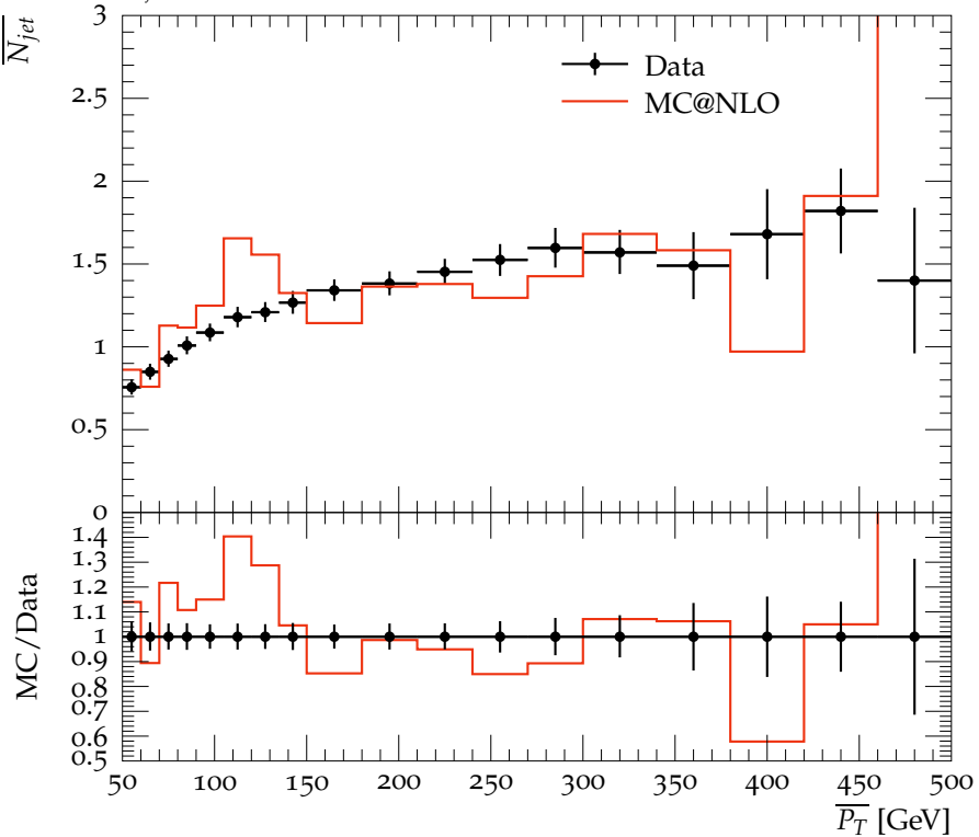
\overline{N}_{jet} vs \overline{P}_T for 3 < |\Delta y| < 4 , Fwd/Bwd
