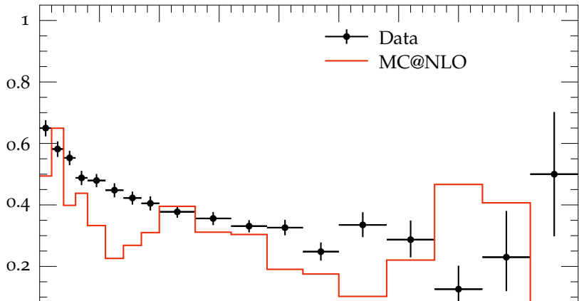
Gap fraction vs \overline{P}_T for 3.0 < |\Delta y| < 4.0 , Leading Jet
