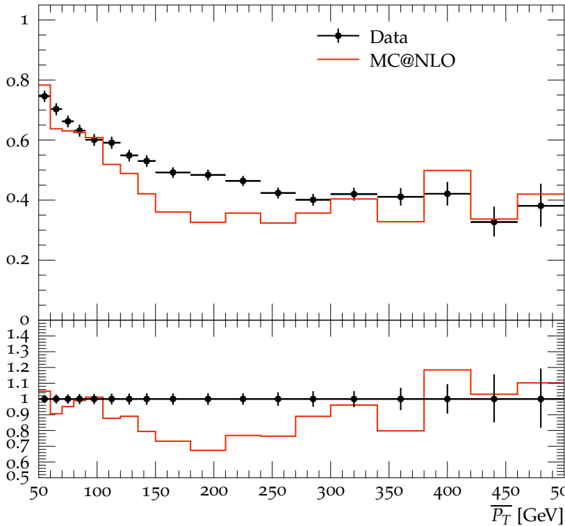
Gap fraction vs \overline{P}_T for 2.0 < |\Delta y| < 3.0 , Leading Jet
