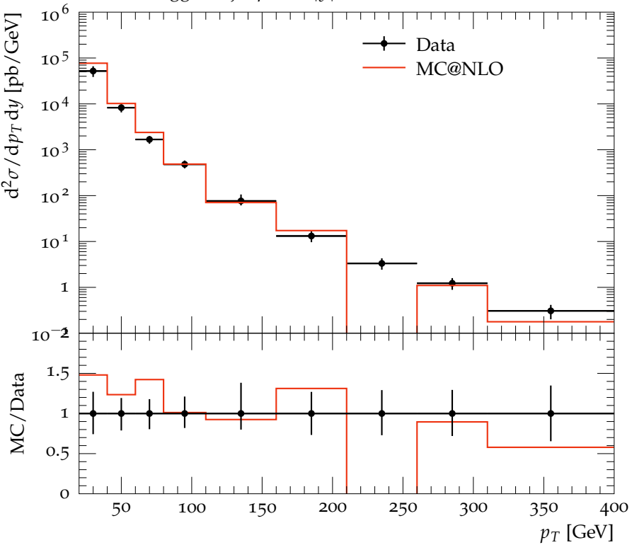
Lifetime tagged b -jet p_T for |y| < 0.3 , anti- k_T , R = 0.4
