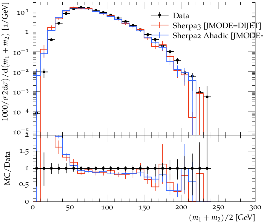
Ungroomed AK7 dijets, (p_T^1 + p_T^2)/2 = 500\text{--}600 GeV
