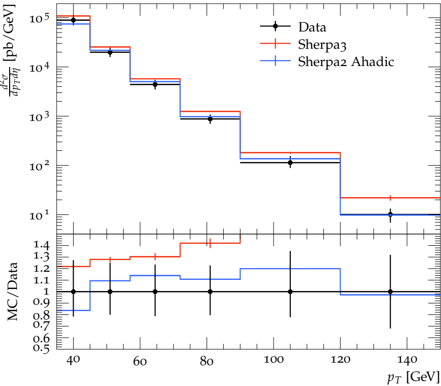
Measurement of forward jets in pp collisions at \sqrt{s} = 7 TeV
