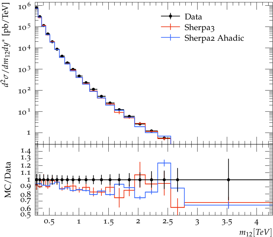
Dijet double-differential cross sections ( y^* < 0.5 ), R=0.4
