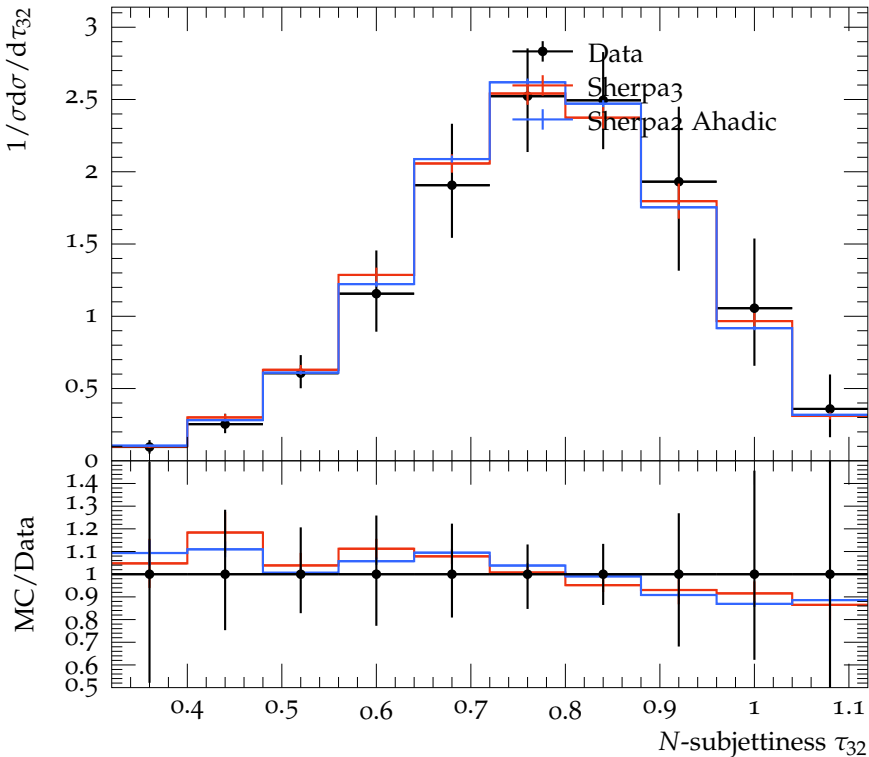
Cambridge-Aachen jets, R=1.2 , 400 \text{ GeV} < p_{\perp} < 500 \text{ GeV}
