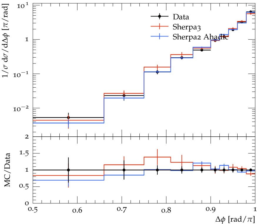
Dijet azimuthal decorrelations for 400 < p_{\perp}^{\text{max}}/\text{GeV} < 500
