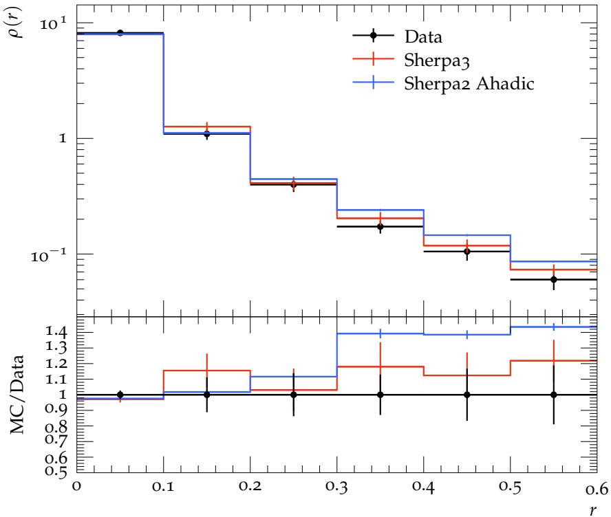
Jet shape \rho for p_{\perp} \in 400\text{--}500 GeV, y \in 1.2\text{--}2.1
