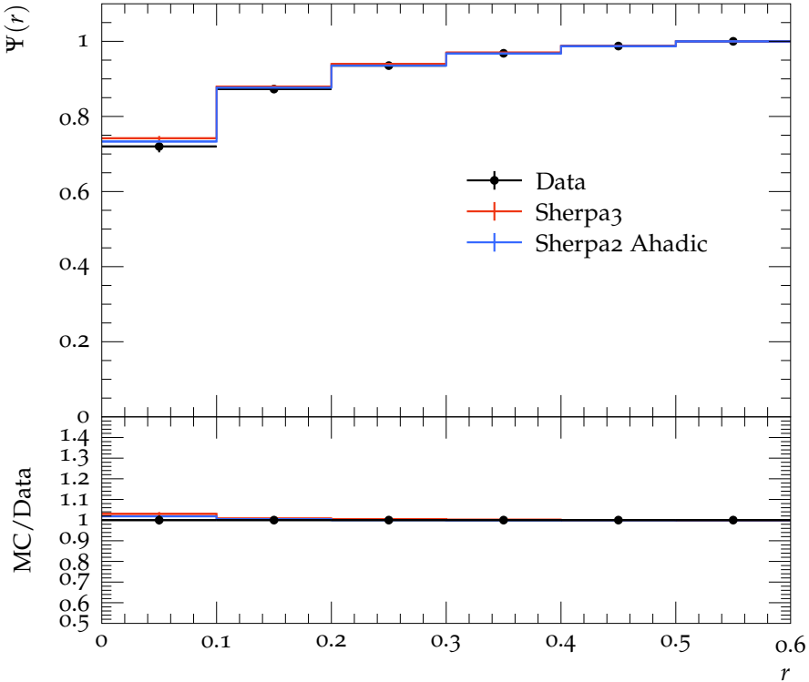
Jet shape \Psi for p_{\perp} \in 210\text{--}260\text{ GeV} , y \in 1.2\text{--}2.1
