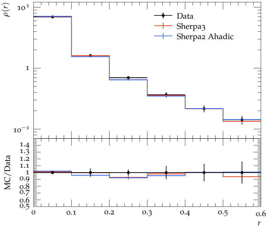
Jet shape \rho for p_{\perp} \in 210\text{--}260 GeV, y \in 0.8\text{--}1.2
