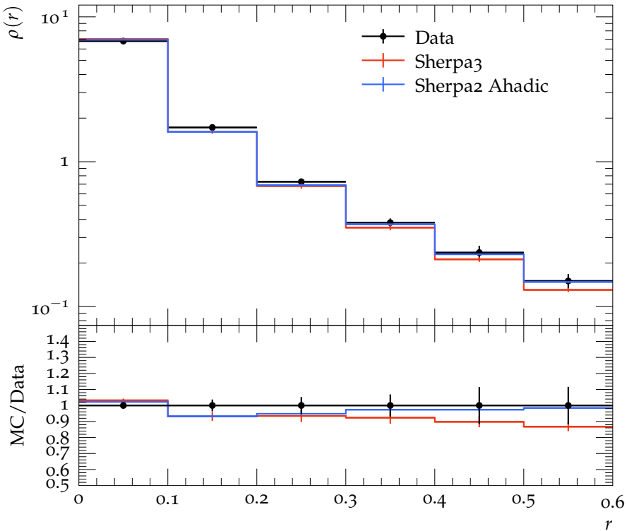
Jet shape \rho for p_{\perp} \in 210\text{--}260 GeV, y \in 0.0\text{--}0.3
