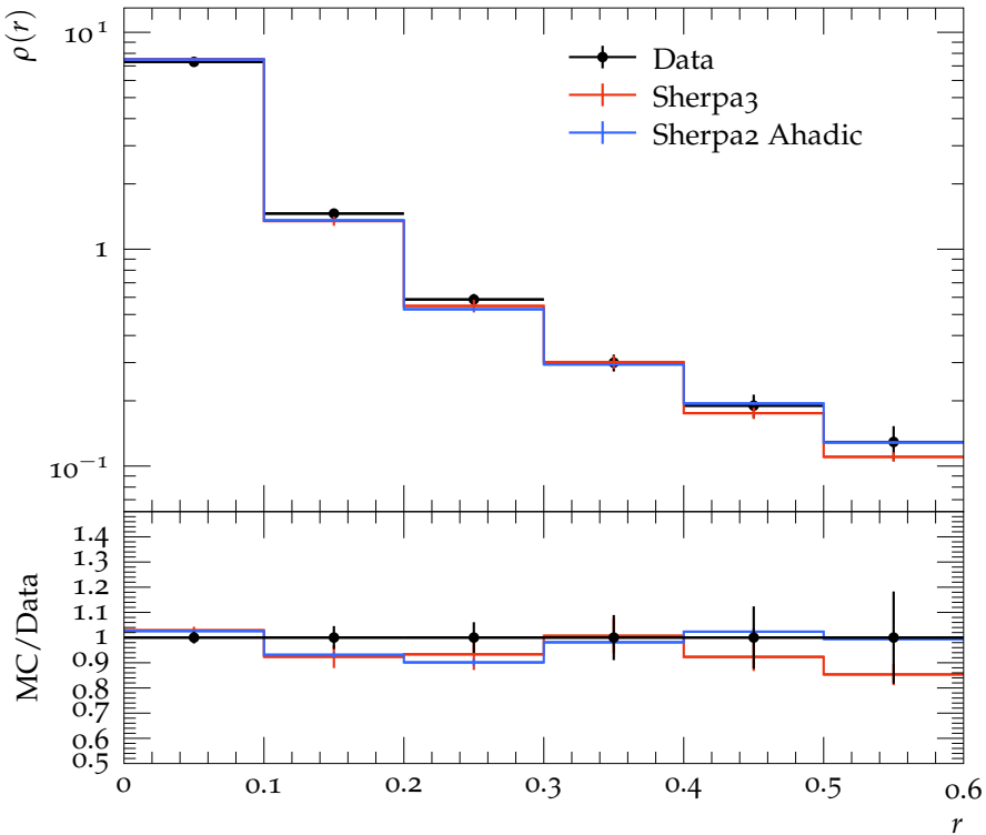
Jet shape \rho for p_{\perp} \in 160\text{--}210 GeV, y \in 2.1\text{--}2.8
