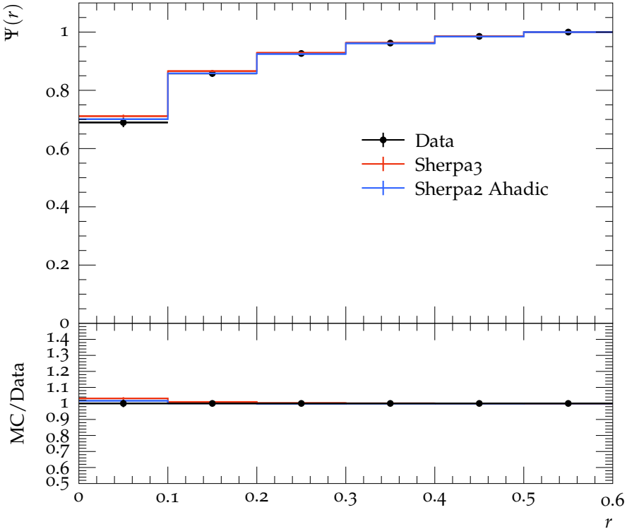
Jet shape \Psi for p_{\perp} \in 160\text{--}210\text{ GeV} , y \in 1.2\text{--}2.1
