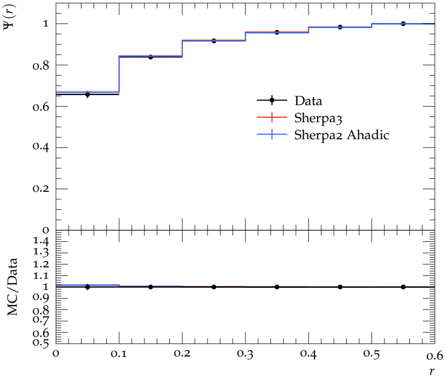
Jet shape \Psi for p_{\perp} \in 160\text{--}210\text{ GeV} , y \in 0.0\text{--}0.3
