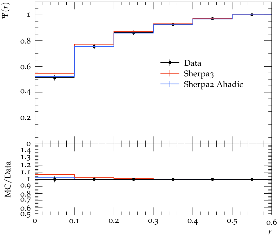
Jet shape \Psi for p_{\perp} \in 60\text{--}80\text{ GeV} , y \in 0.3\text{--}0.8
