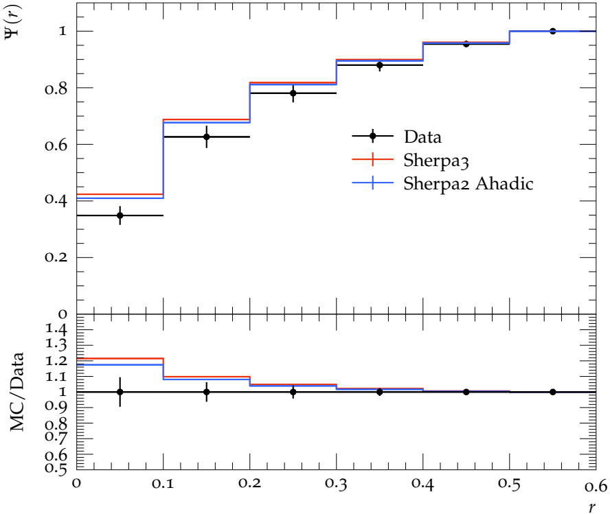
Jet shape \Psi for p_{\perp} \in 30\text{--}40\text{ GeV} , y \in 0.0\text{--}2.8
