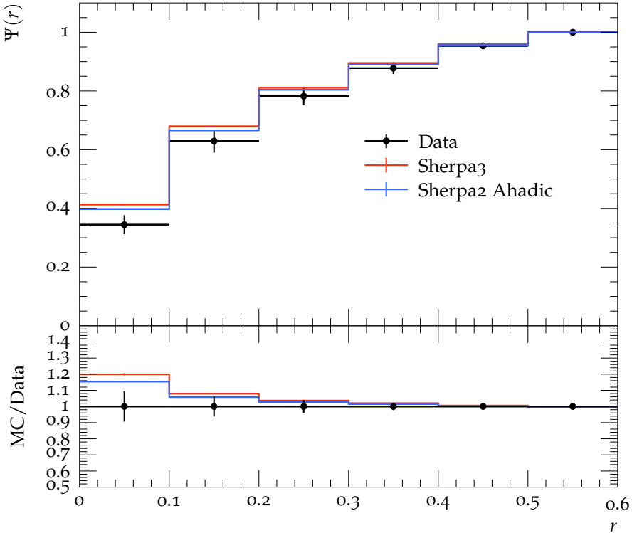
Jet shape \Psi for p_{\perp} \in 30\text{--}40\text{ GeV} , y \in 0.0\text{--}0.3
