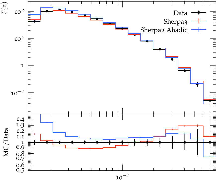
F(z) for 25 \text{ GeV} < p_{T \text{ jet}} < 40 \text{ GeV}
