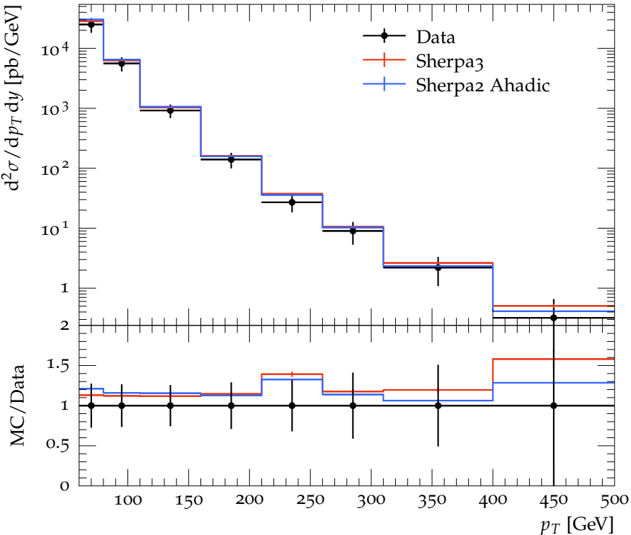
Inclusive jet p_T spectrum for 1.2 < |y| < 2.1 . anti-KT, R = 0.4 .
