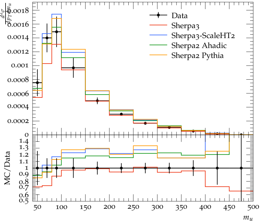
CMS, 13 TeV, Ungroomed jet mass m_u ( 900 < p_T < 1000 GeV)
