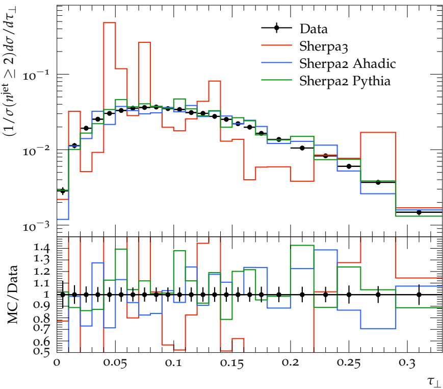
Transverse Thrust for n^{\text{jet}} \geq 6 , 1.5 \text{ TeV} < H_{T2} < 2.0 \text{ TeV}
