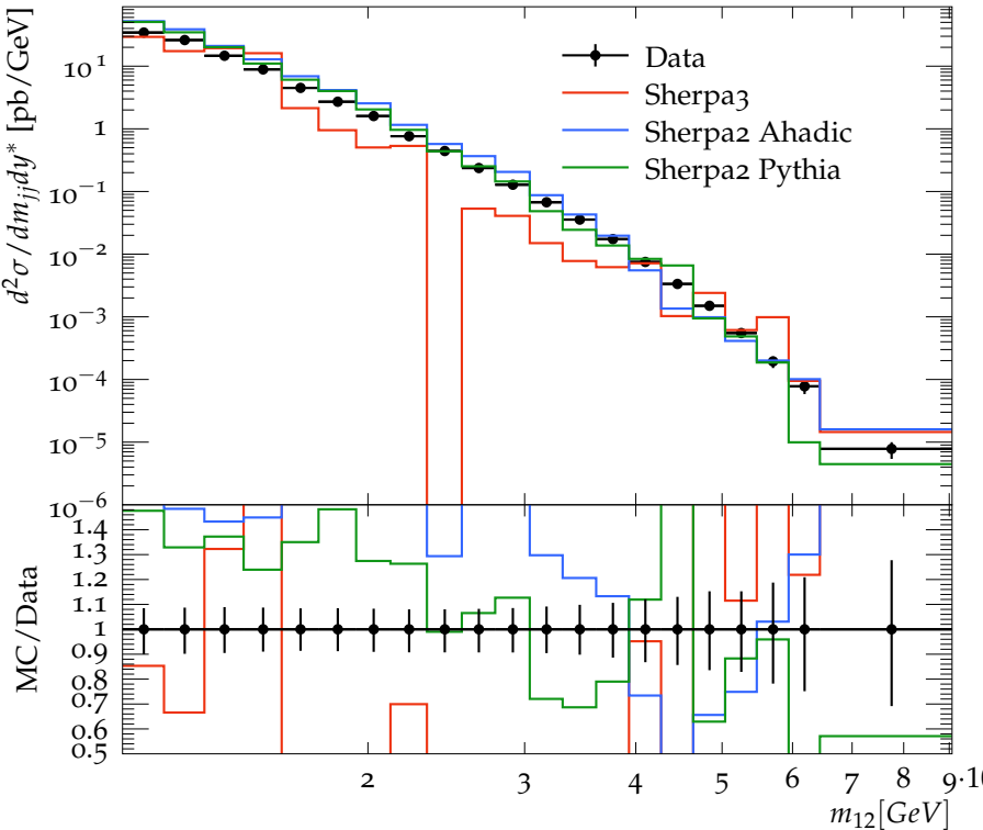
Dijet cross section ( 2.0 \leq y^* < 2.5 ), R=0.4
