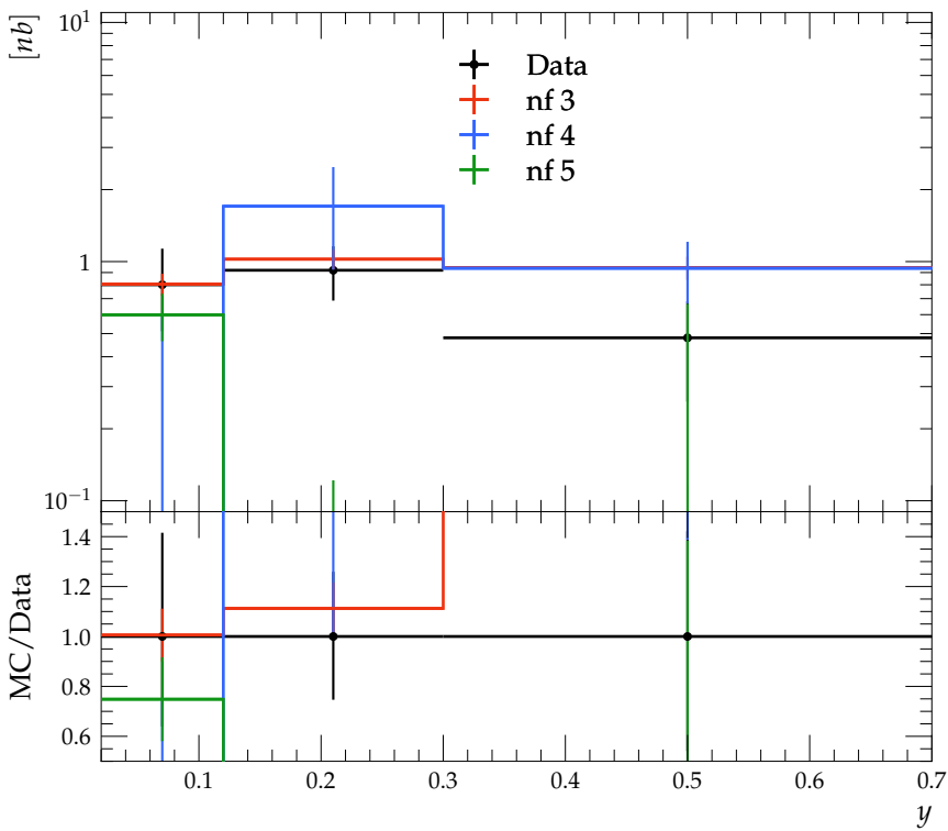
Differential cross-section of D^0 meson production for 5.0 < Q^2 < 9.0
