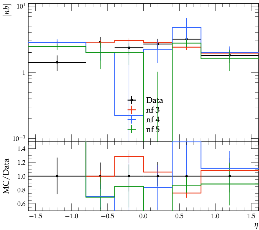
Differential cross-section of D^0 meson production
