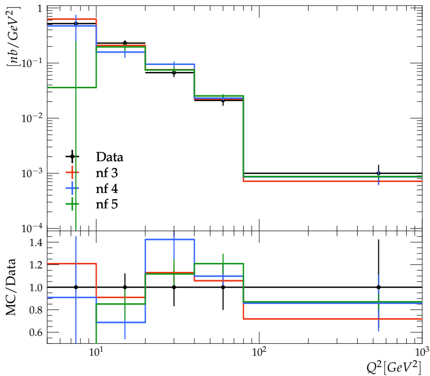
Differential cross-section of D^0 meson production
