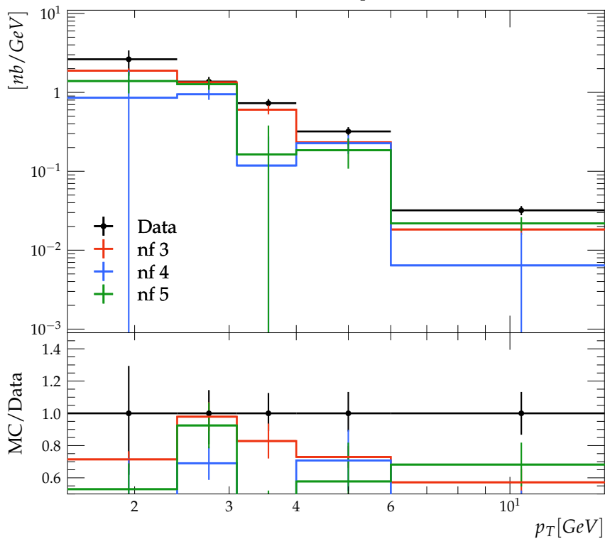
Differential cross-section of D^\pm meson production
