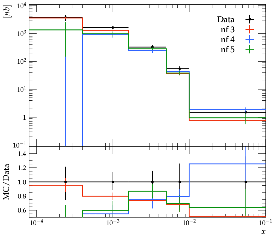
Differential cross-section of D^\pm meson production
