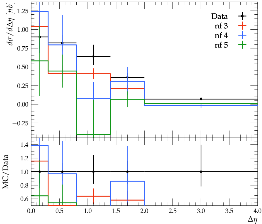
d\sigma/d\Delta\eta for D^{*\pm} production with dijets
