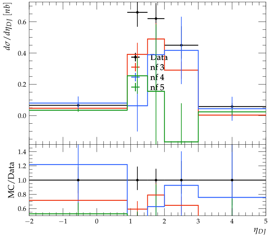
d\sigma/d\eta_{DJ} for D^{*\pm} production with dijets
