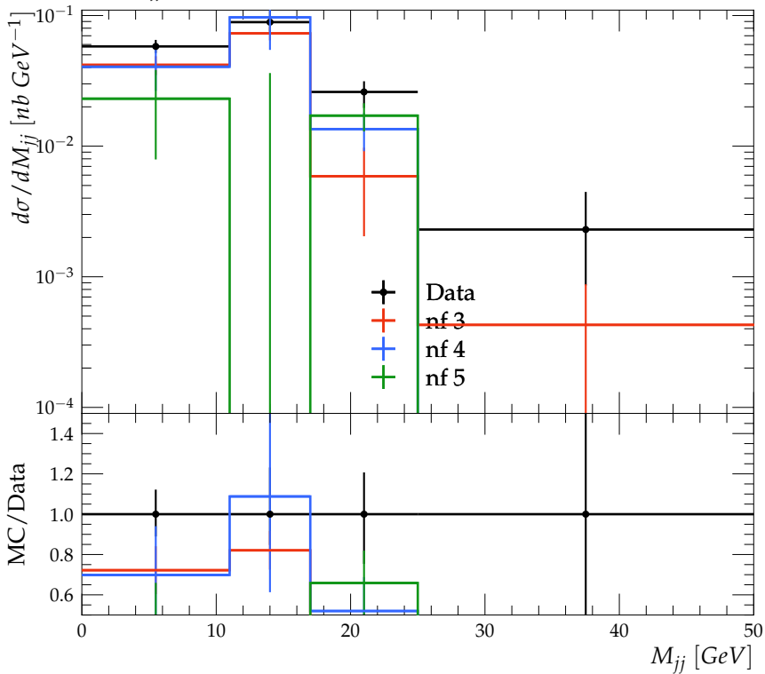
d\sigma/dM_{jj} for D^{*\pm} production with dijets (Breit frame)
