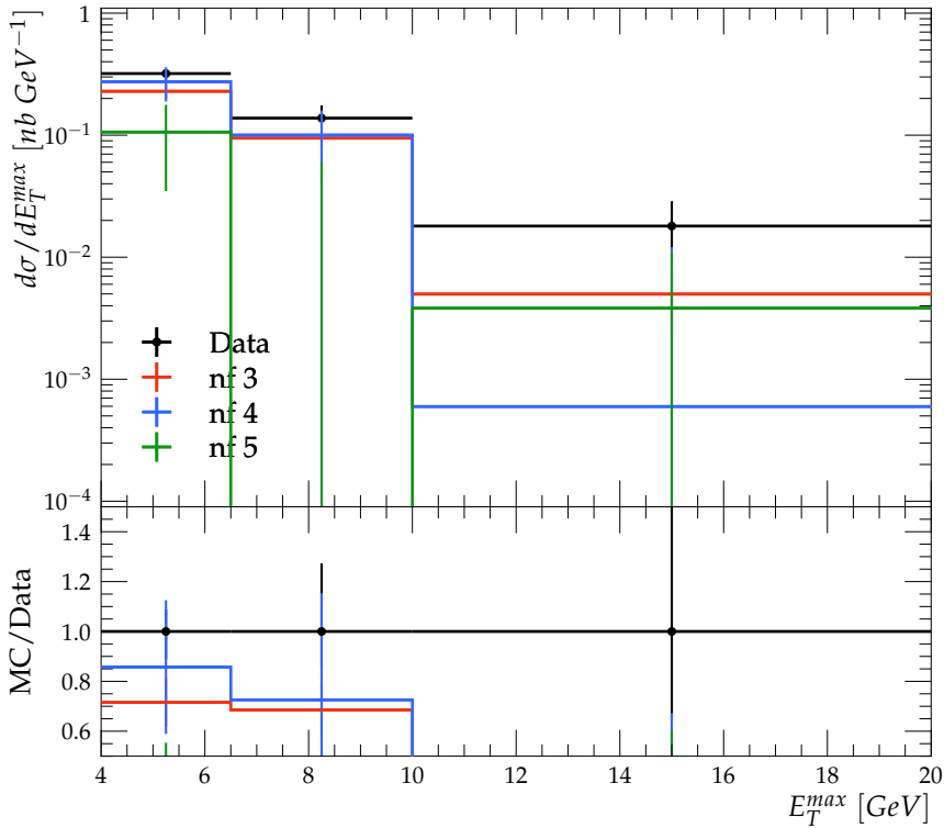
d\sigma/dE_T^{max} for D^{*\pm} production with dijets (Breit frame)
