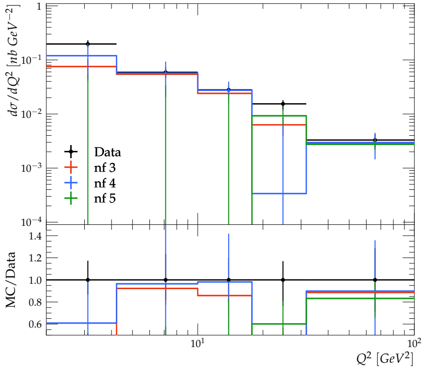
d\sigma/dQ^2 for D^{*\pm} production with dijets (Breit frame)
