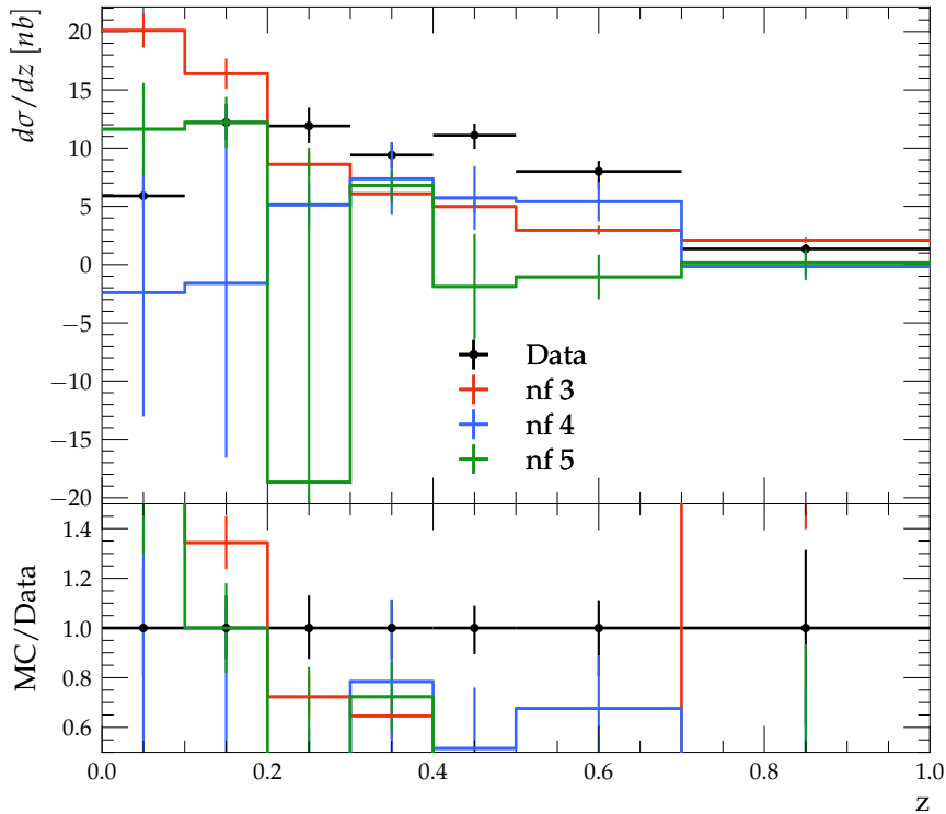
d\sigma/dz for inclusive D^{*\pm} production in the vis. kin. region
