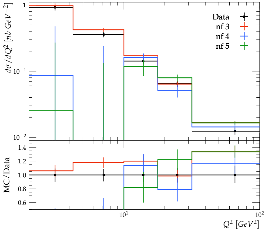
d\sigma/dQ^2 for inclusive D^{*\pm} production in the vis. kin. region
