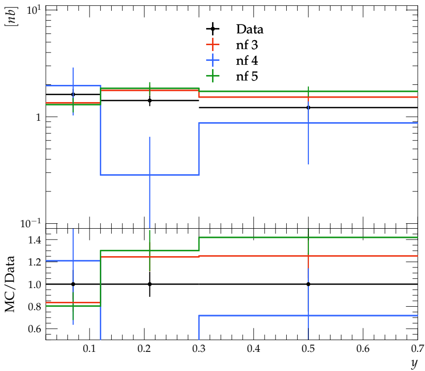
Differential cross-section of D^0 meson production for 9.0 < Q^2 < 44.0
