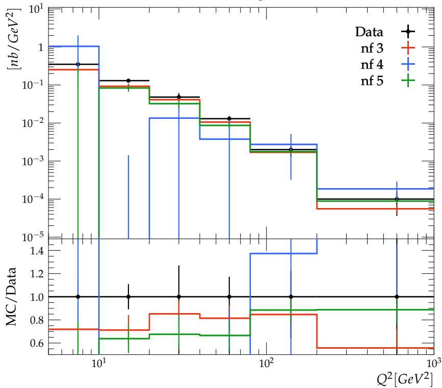
Differential cross-section of D^\pm meson production
