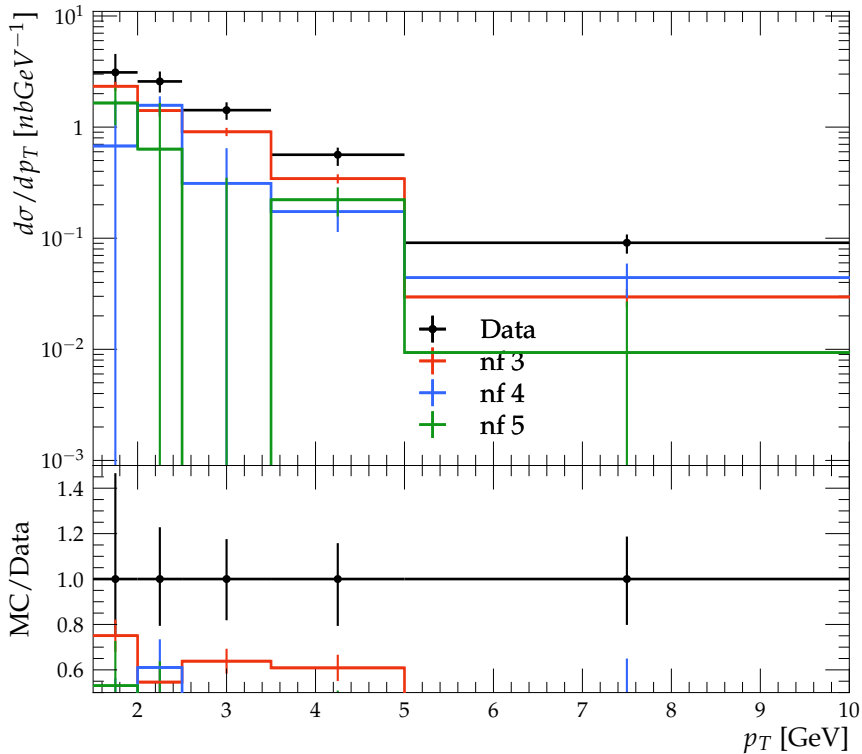
Transverse D* momentum lab frame
