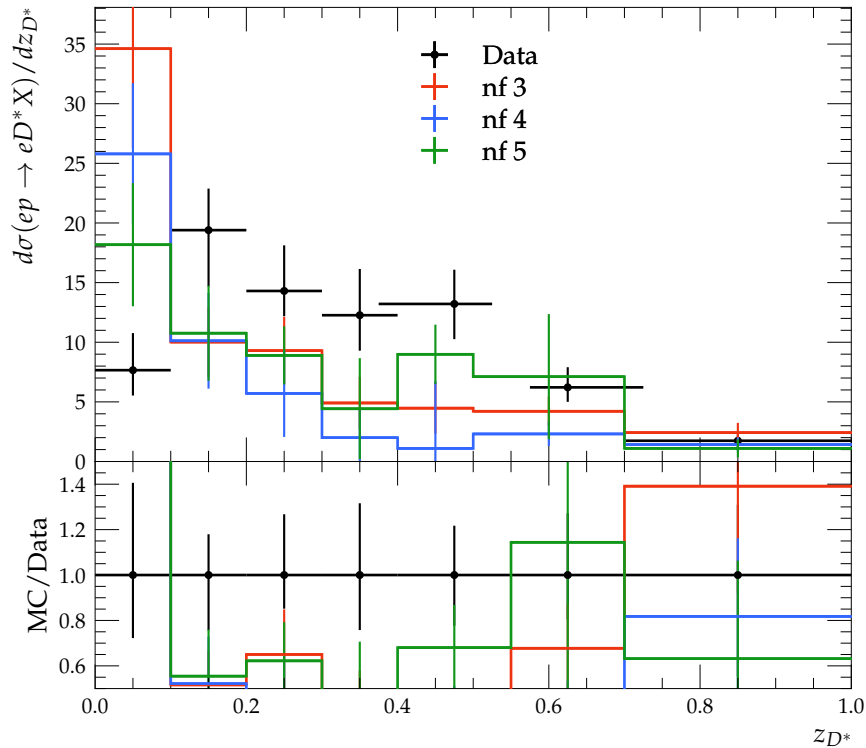
D^* production in DIS (H1)
