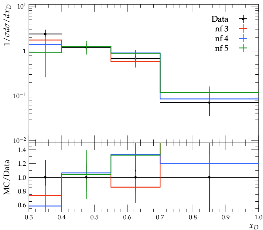
Normalized x_D Distribution for D^0
