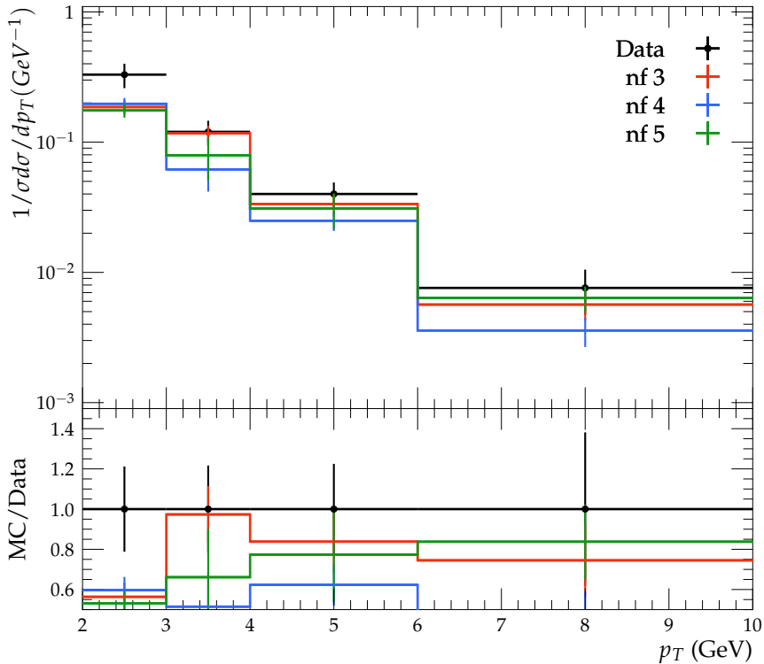
Normalized Differential Cross Section for D^0
