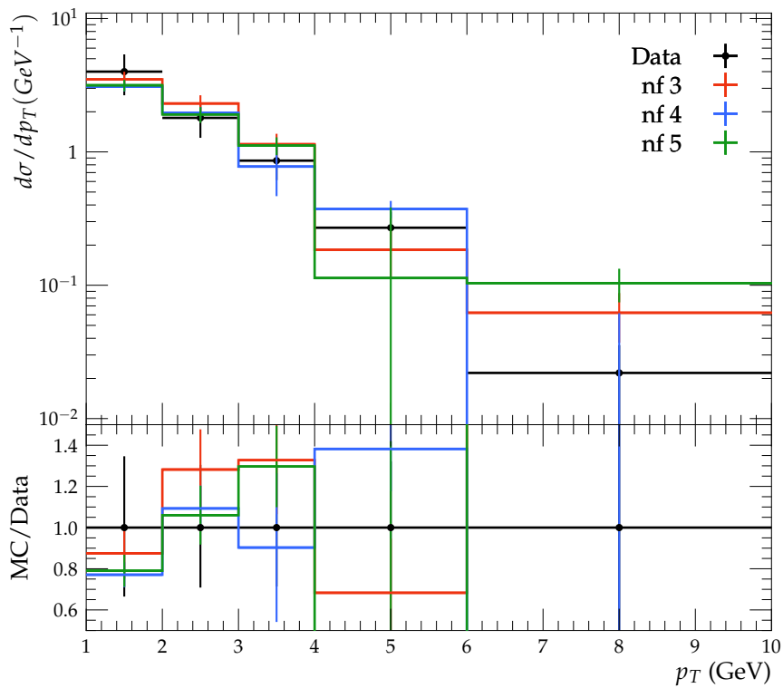
Differential Cross Section for D^*
