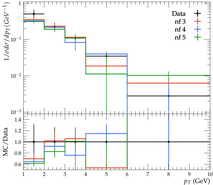
Normalized Differential Cross Section for D^*
