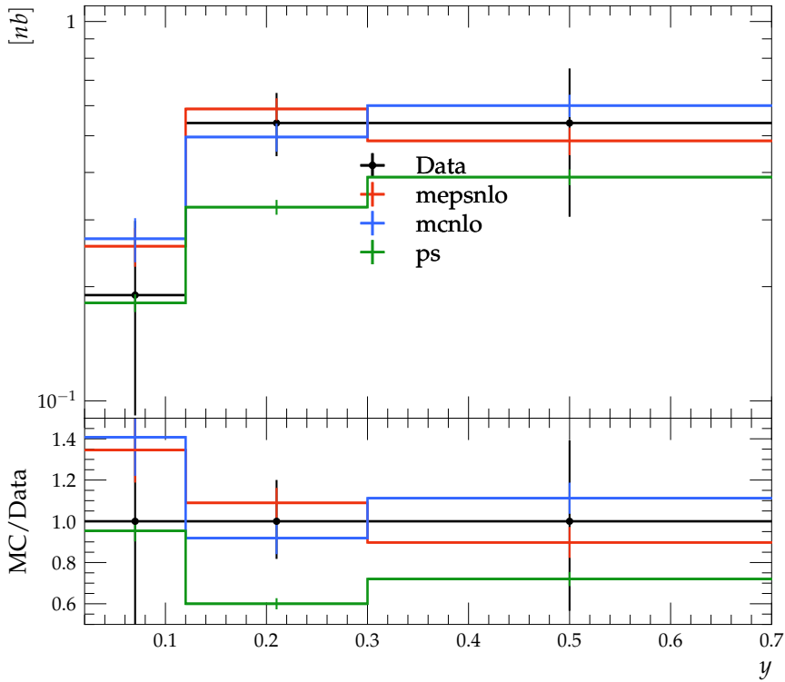
Differential cross-section of D^0 meson production for 44.0 < Q^2 < 1000.0
