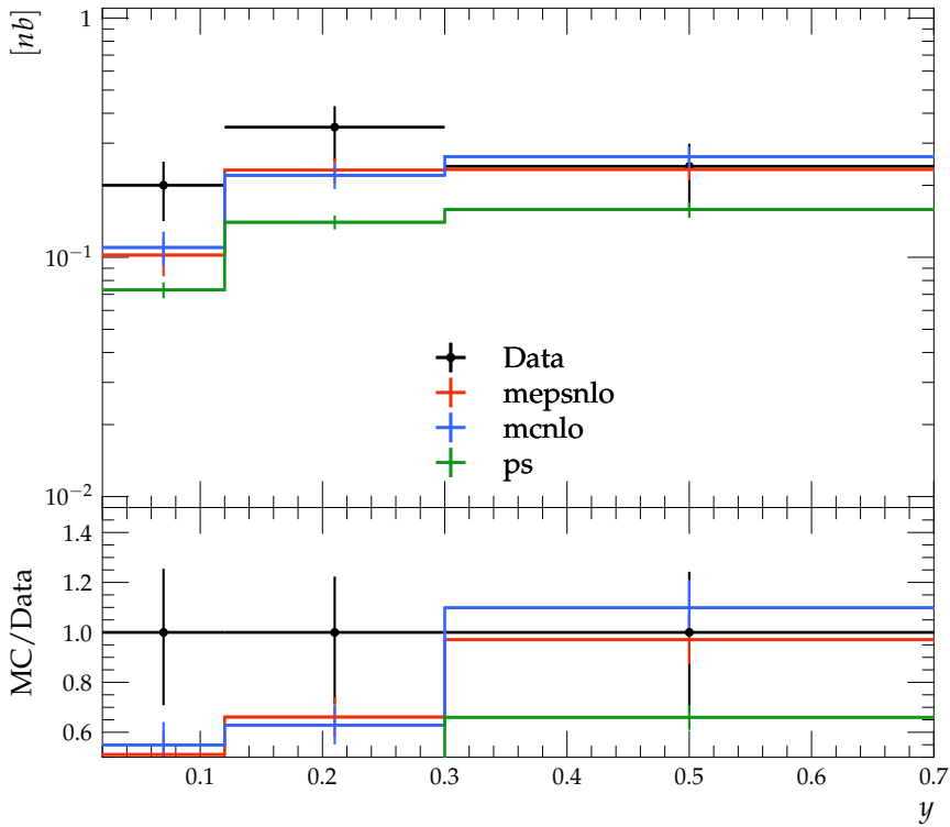
Differential cross-section of D^\pm meson production for 44.0 < Q^2 < 1000.0
